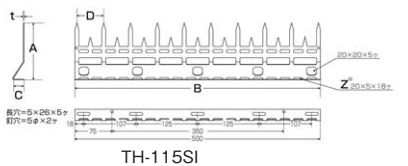
TH-115SI
