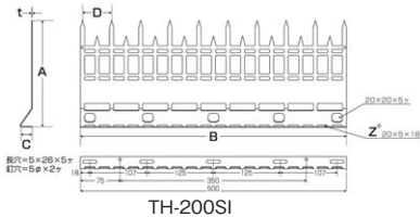
TH-200SI
