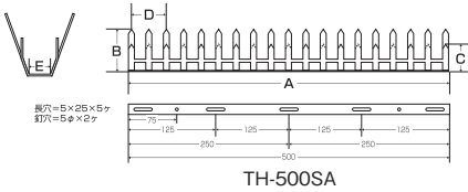
TH-500SA
